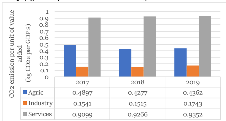
Figure 59: CO 2 emission per unit of value added by sector, 2017-2019 (kg CO 2 e per constant 2010 GDP $)
